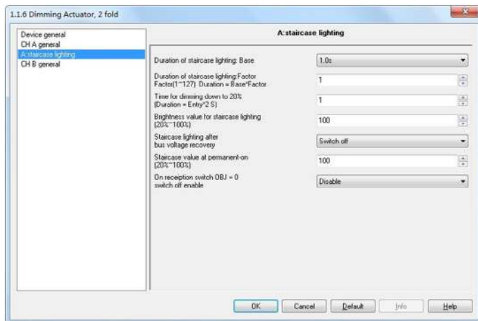
Fig. 6.8 parameter window "CH X staircase lighting"
