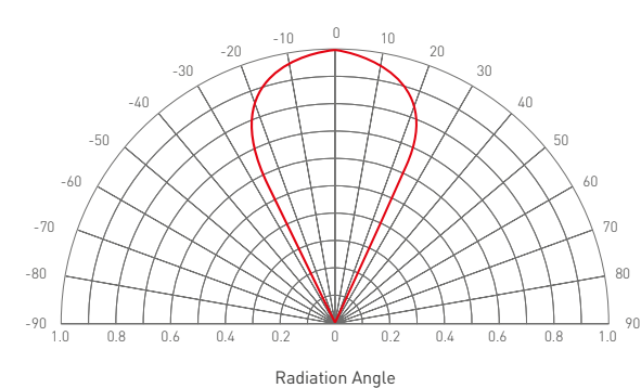
Radiation Characteristics
