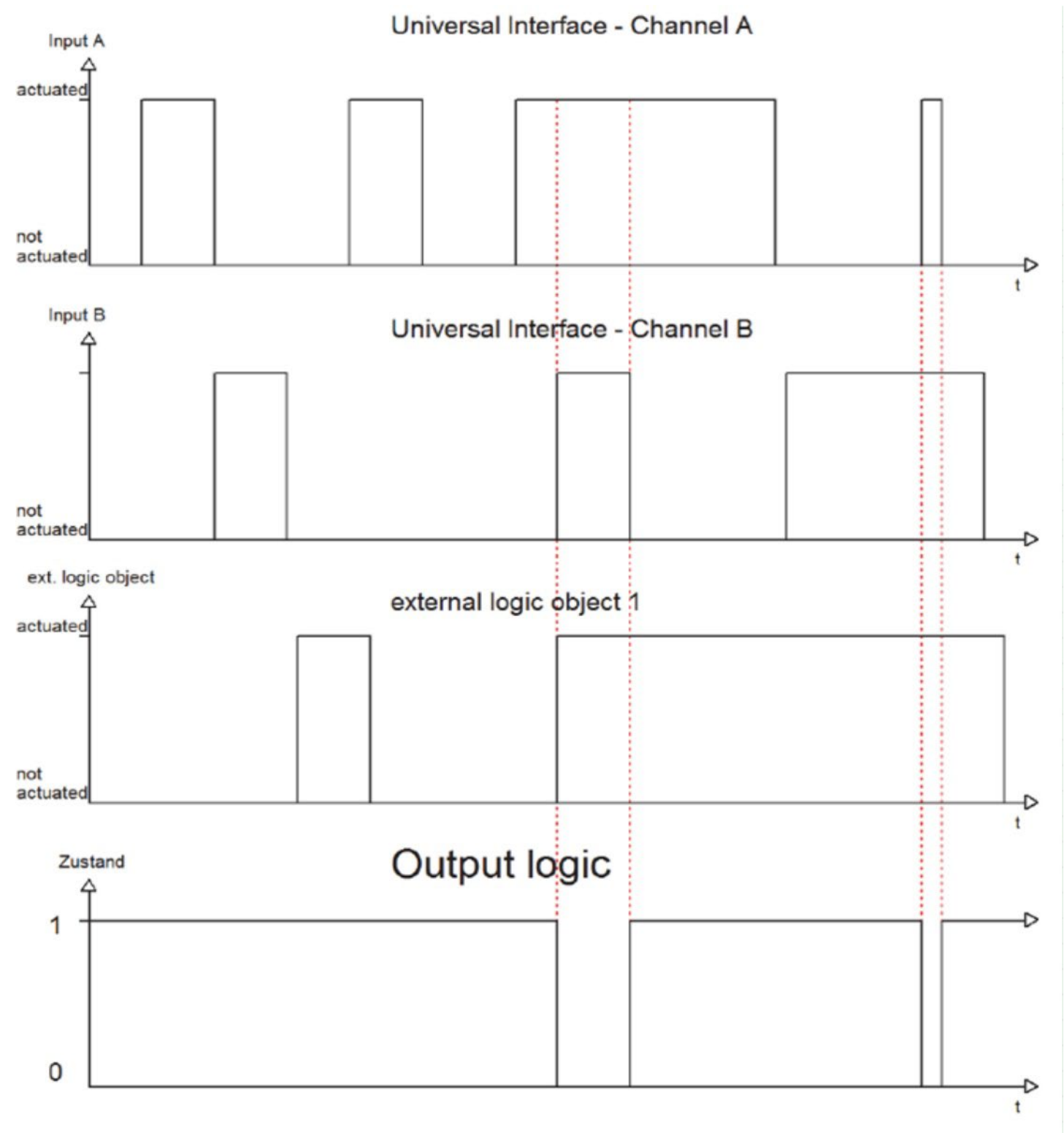
Figure 29: Logic output
