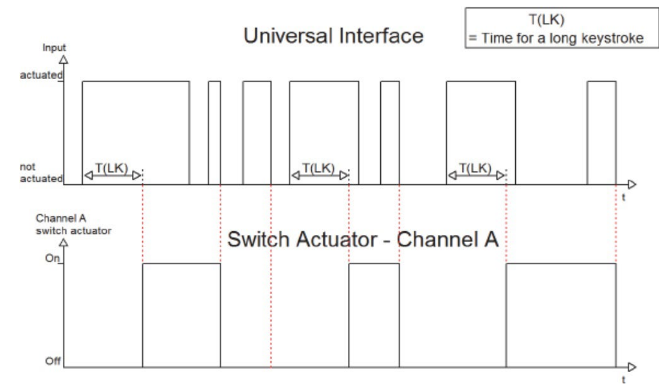
Figure 22: Long/short press together
