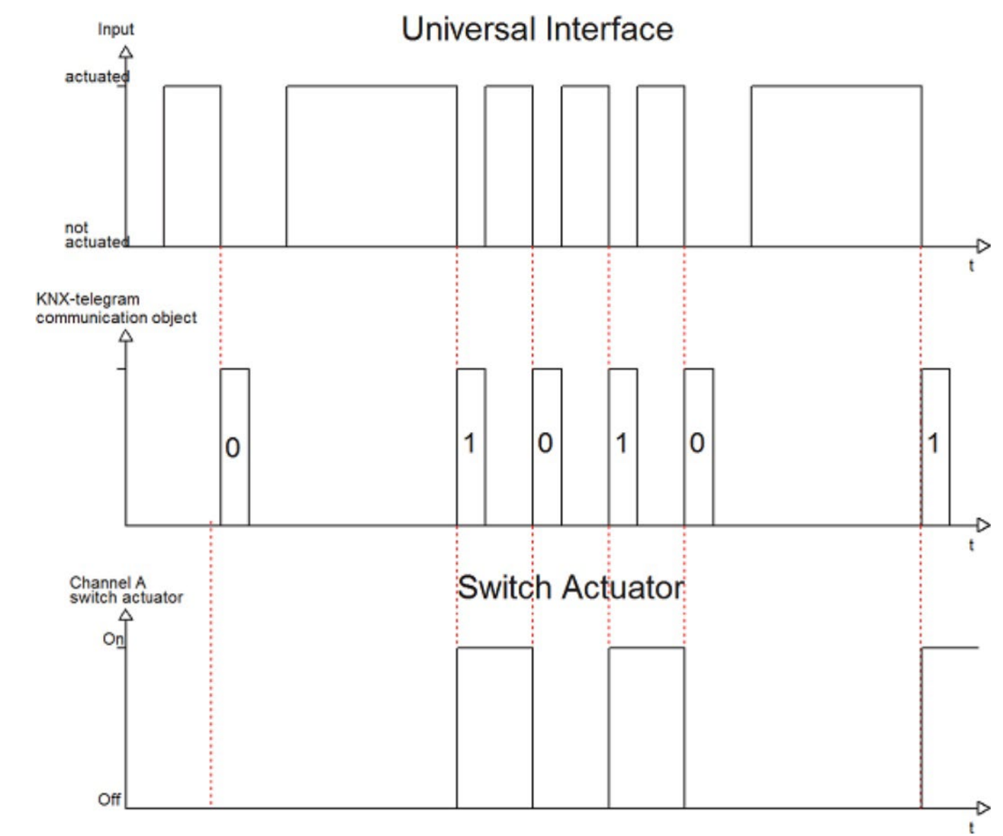
Figure 11: Drop delay flip
