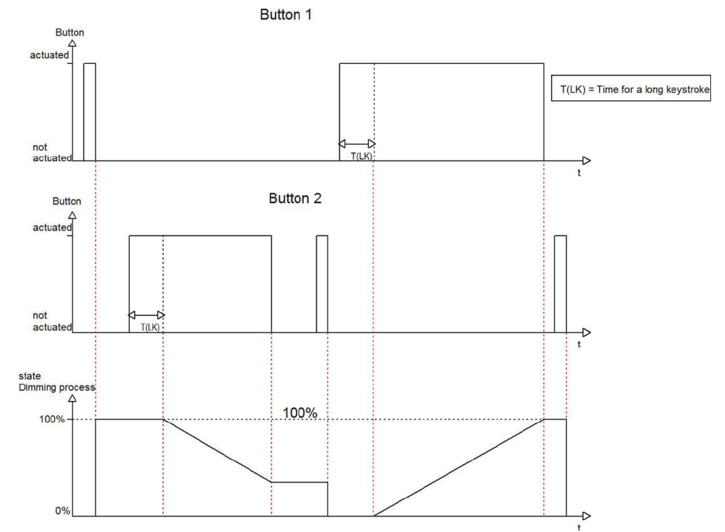
Figure 6: Double key dimming waveform
