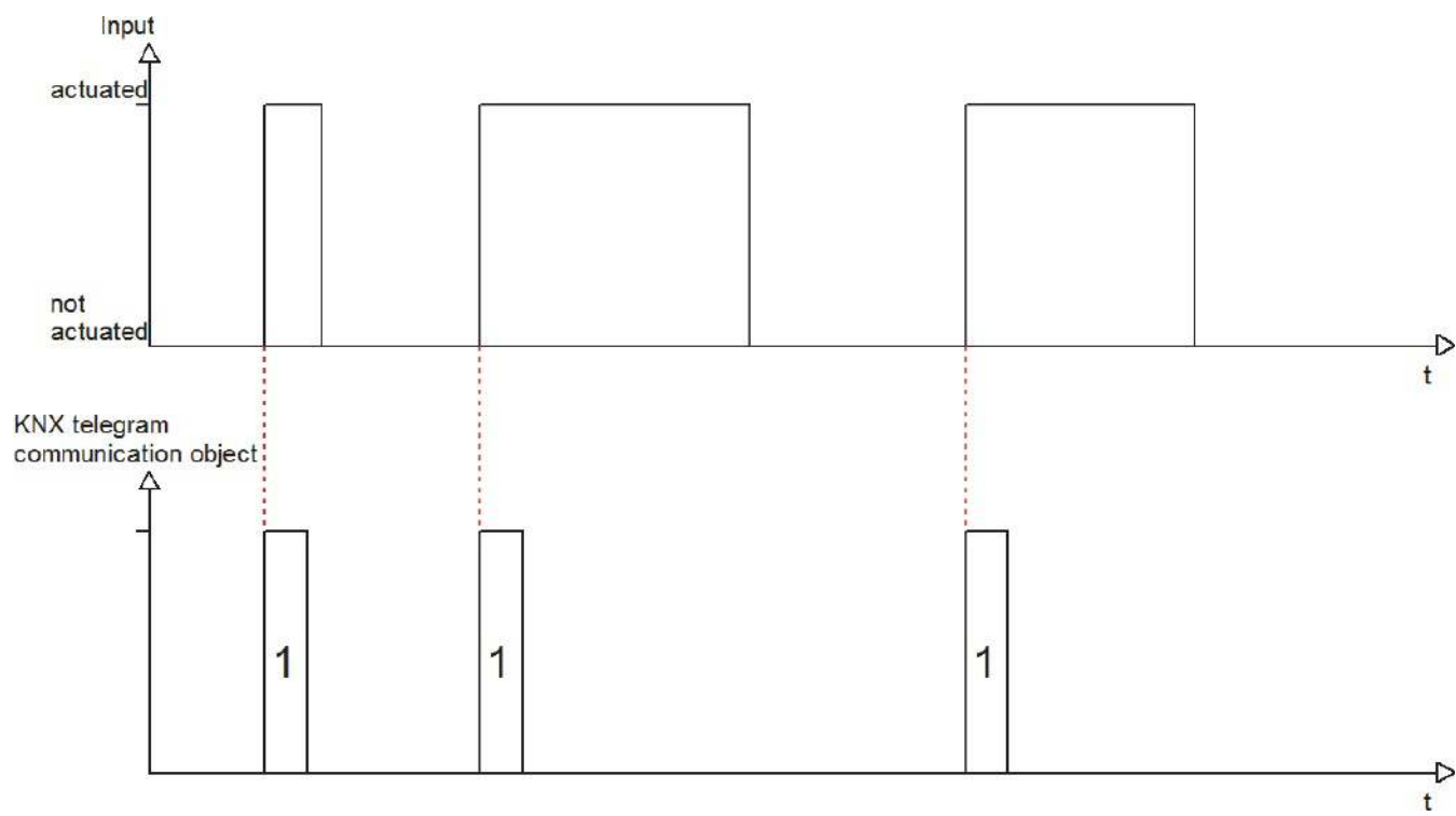
Figure 10: Press to send the On signal
