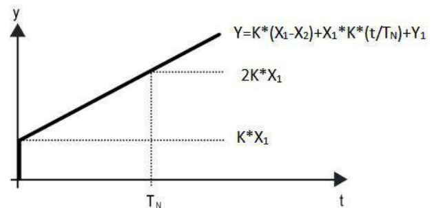
Fig. 1.3.3 (7) control value of PI control mode
